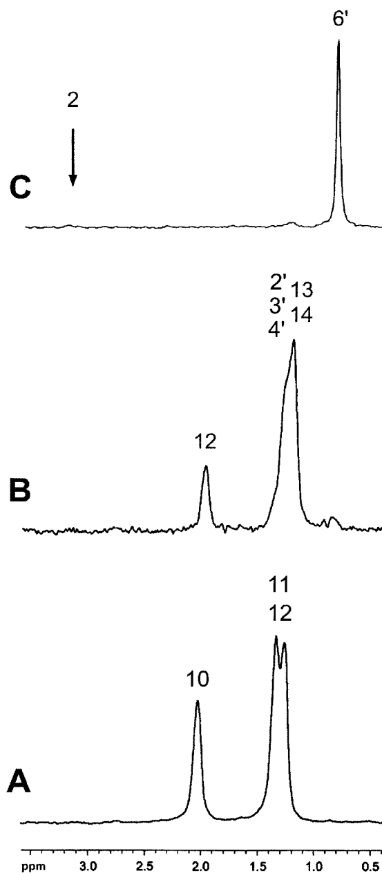
Figure 2. (A) ^2\text{H} NMR signals of (5 Z ,8 Z )-[10,11,12,12- ^2\text{H} ]tetradeca-5,8-dienoic acid ( 13 ). (B) ^2\text{H} NMR signals of lipstatin isolated from a fed-batch culture of S. toxytricini growing with (5 Z ,8 Z )-[10,11,12,12- ^2\text{H} ]tetradeca-5,8-dienoic acid ( 13 ) as supplement. (C) ^2\text{H} NMR signals of lipstatin isolated from a fed-batch culture of S. toxytricini growing with an equimolar mixture of [2,2- ^2\text{H}_2 ]- and [8,8,8- ^2\text{H}_3 ]octanoic acid as supplement. The arrow points to the position of the absent deuterium signal at C-2 (for details see text).
